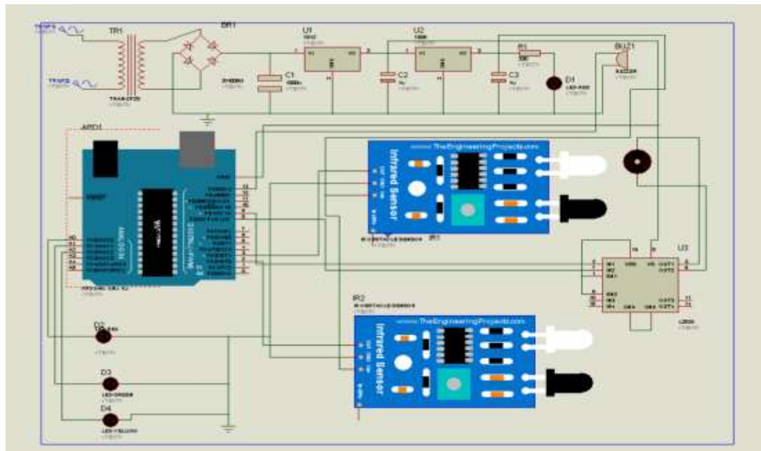
Figure.2 Schematic Diagram
