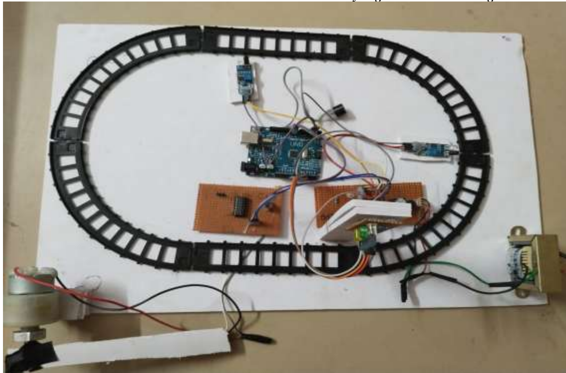
Figure.3 Working Kit
