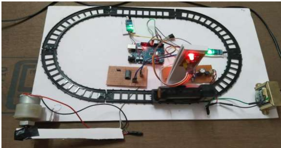
Figure.4 Testing
