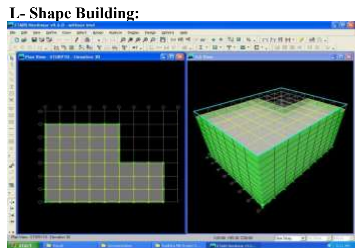
Fig.5. Unsymmetrical Building Plan without TMD.
