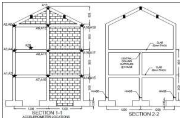
Figure 2: Accelerometer locations for the 3D-RC Structure
