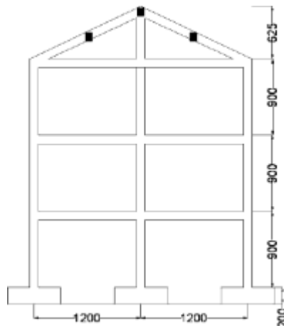
Figure 1: Dimensions of Model of a 3D-RC Structure
