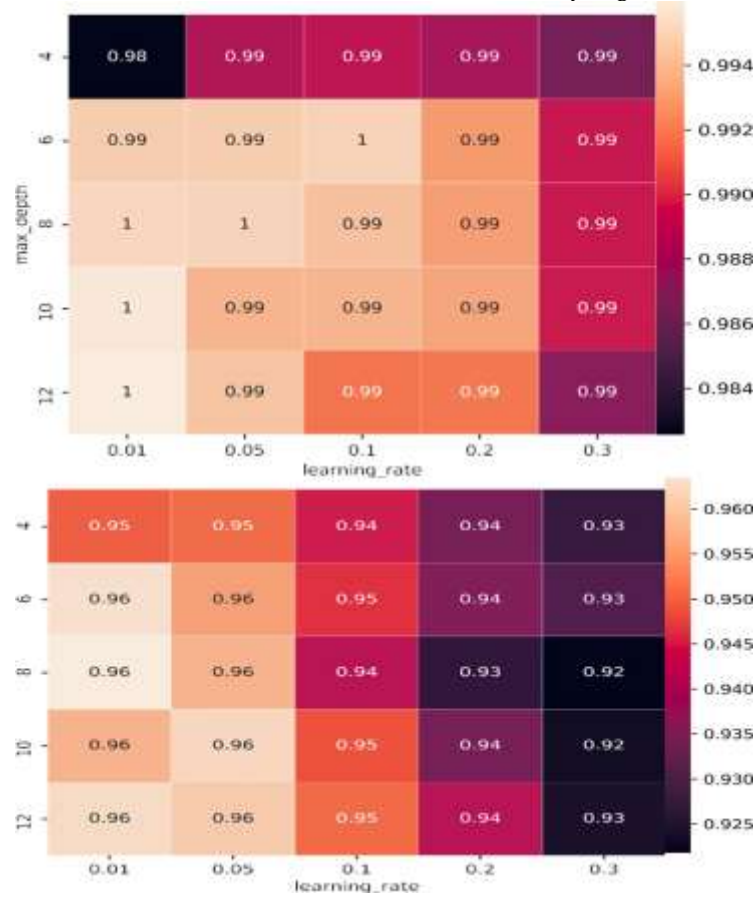
Hyperparameters for XG Boost and CatBoost algorithms
