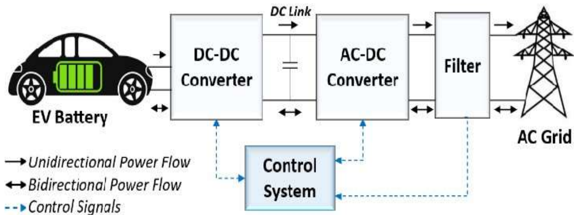
Fig: 1. Block diagram of Fast Charging EV Station
